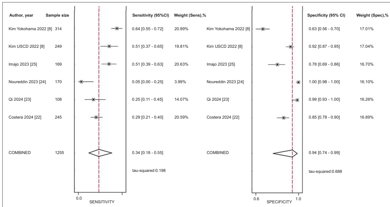
Figure 2 Coupled forest plot of sensitivity and specificity of MEFIB index for ruling in at-risk MASH
