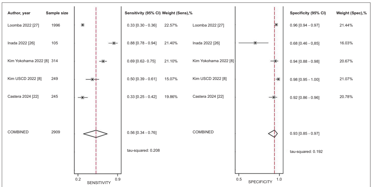
Figure 3 Coupled forest plot of sensitivity and specificity of the MEFIB index for ruling in significant fibrosis
