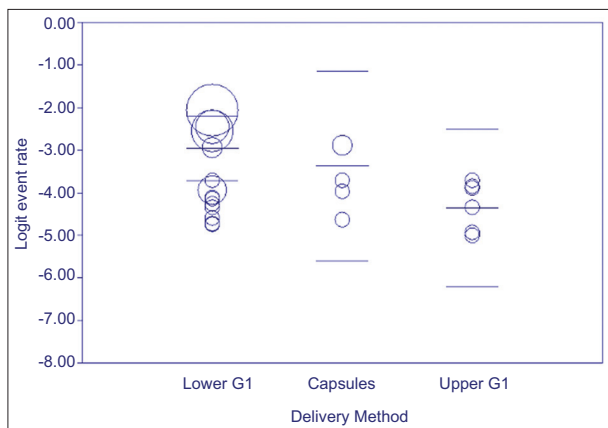
Figure 5 Regression analysis of impact of delivery method on logit of serious adverse event rate*
