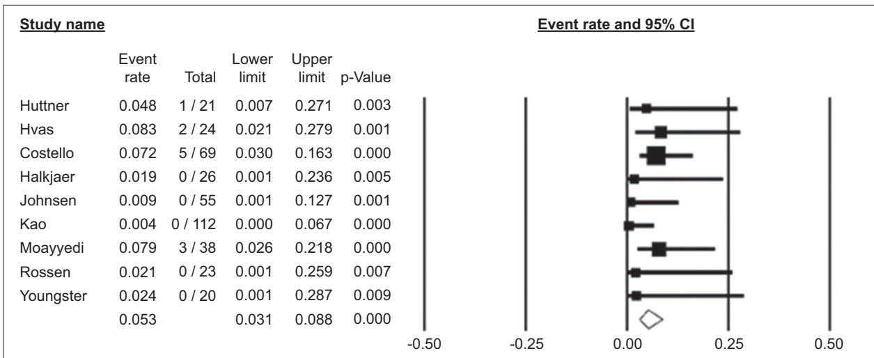
Figure 3 Forest plot of serious adverse event rate CI, confidence interval
