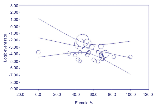
Figure 6 Regression analysis of impact of patient gender on logit of serious adverse event rate*
