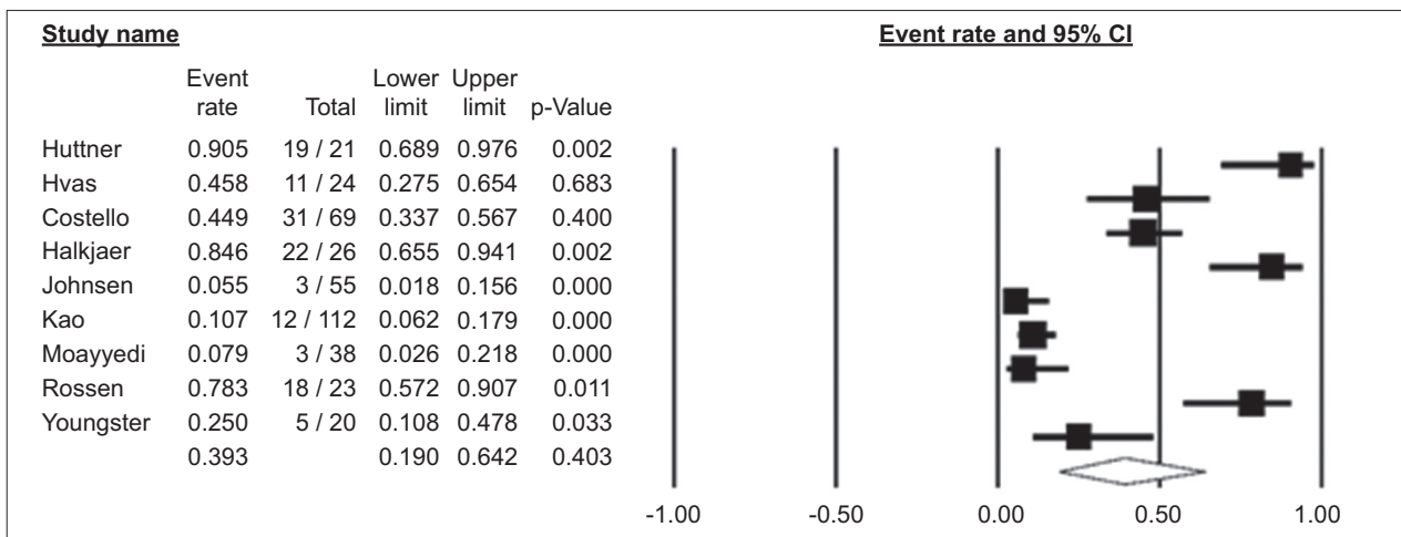
Figure 2 Forest plot of total adverse event rate CI, confidence interval
