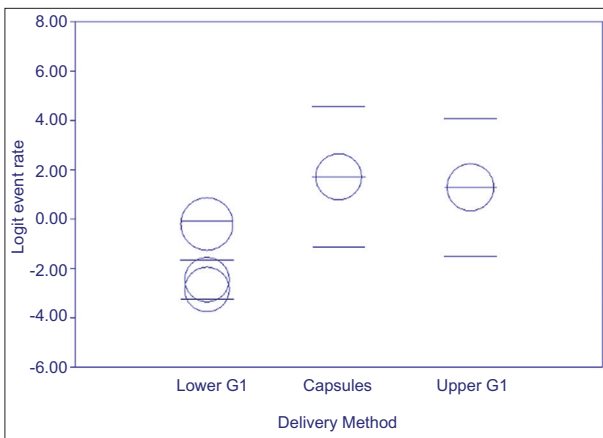
Figure 4 Regression analysis of impact of delivery method on logit of total adverse event rate* *Based on data of from 5 studies from included in the original analysis G1, gastrointestinal
